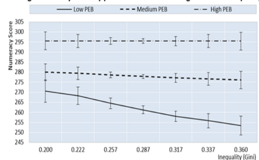
3. Average numeracy score by parent educational background and inequality
